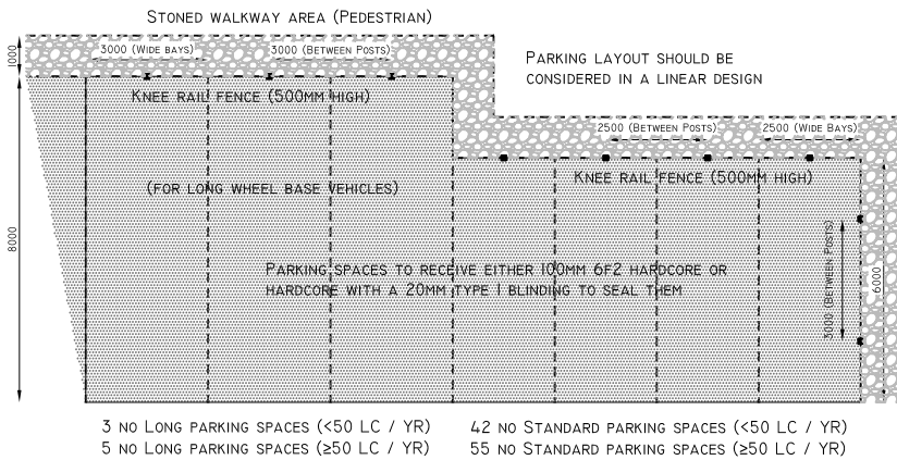
CARPAK LAYOUT
