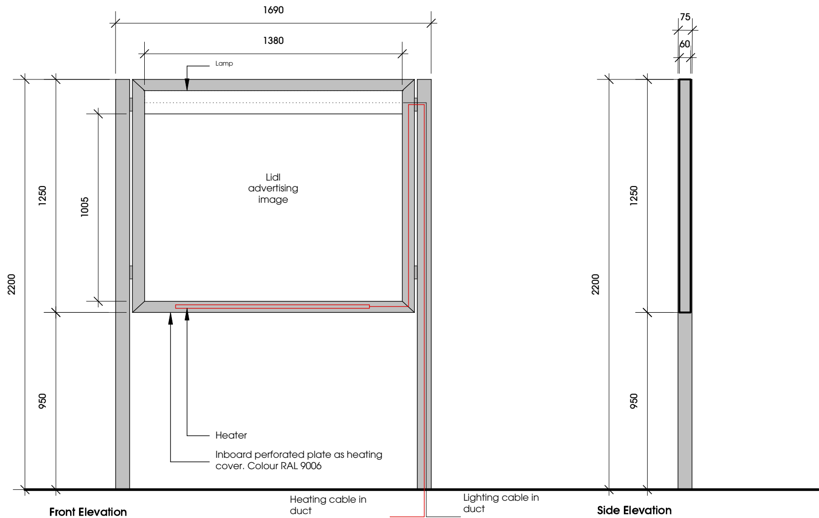
Front Elevation
