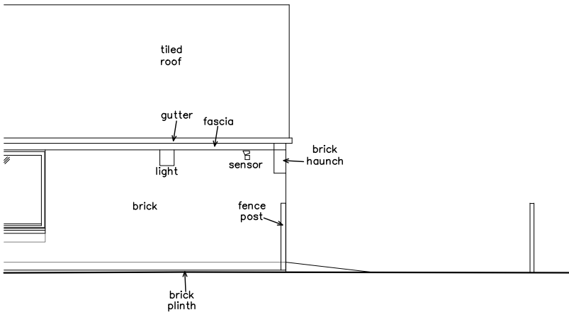
NORTH EAST ELEVATION - SOUTHERN END
