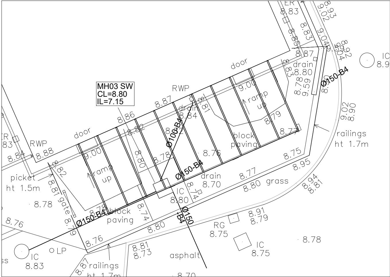
CANOPY B PROPOSED PLAN
