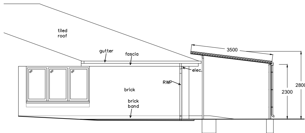
PROPOSED SOUTH WEST ELEVATION
