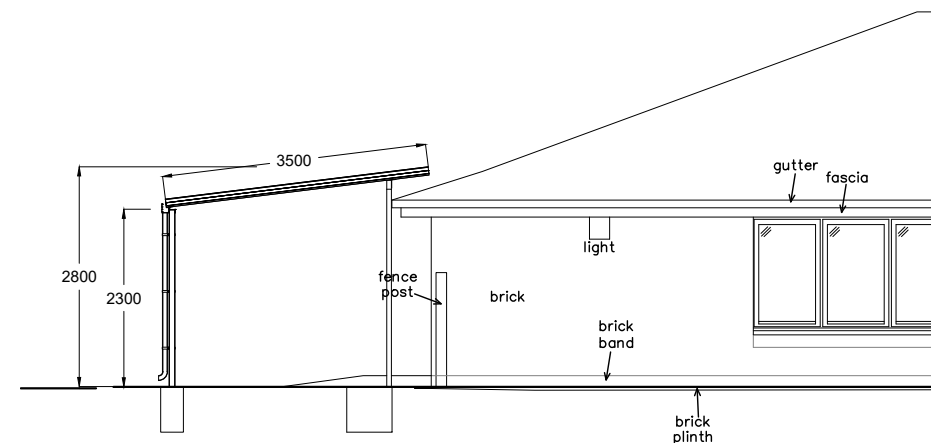
PROPOSED NORTH EAST ELEVATION - SOUTHERN END
