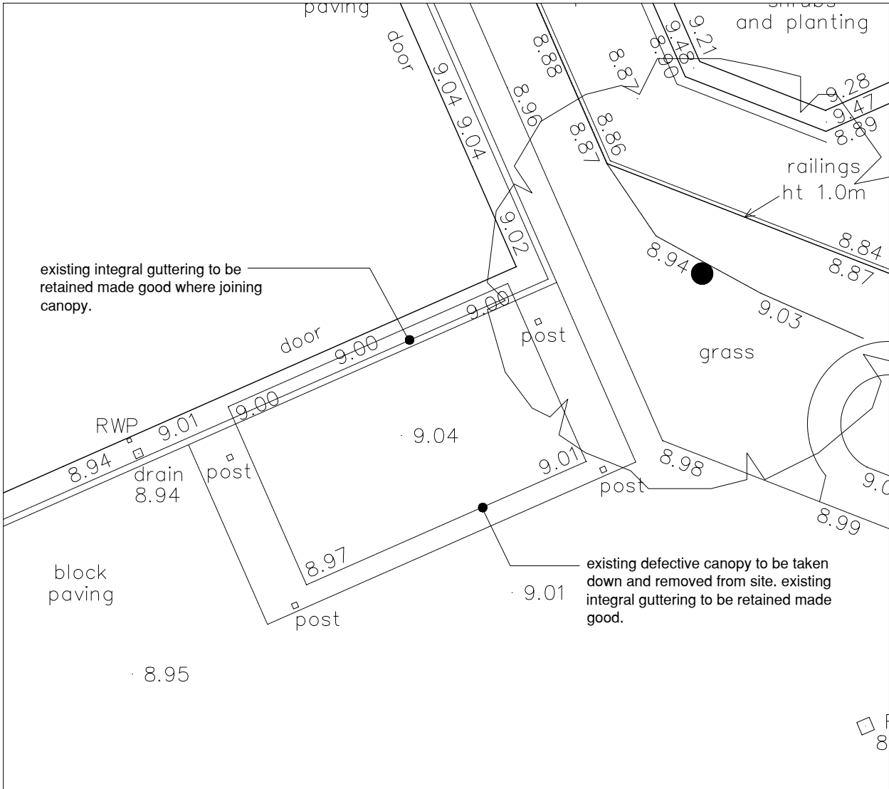
CANOPY C EXISTING PLAN
