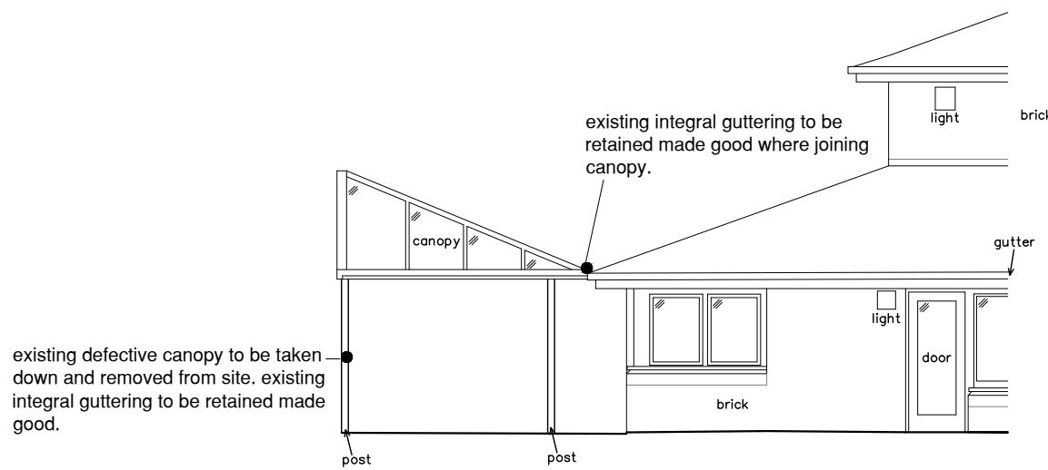
EXISTING ENTRANCE APPROACH SOUTH WEST SIDE
