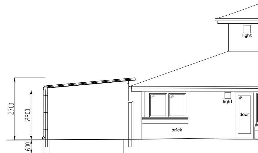
PROPOSED ENTRANCE APPROACH SOUTH WEST SIDE
