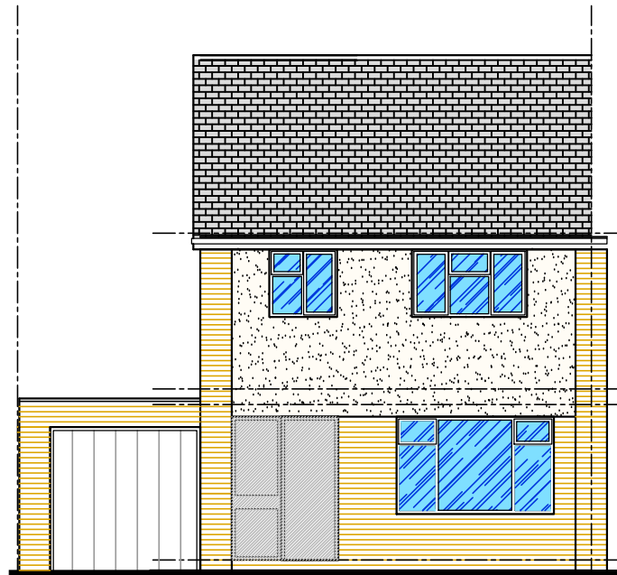
FRONT ELEVATION AS EXISTING
