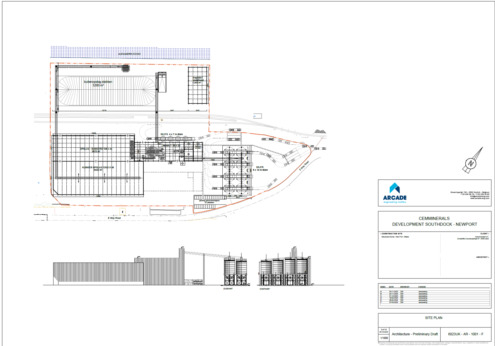
Figure C 2 Proposed site layout
