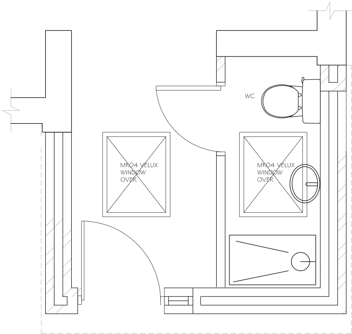
Proposed Front porch layout
