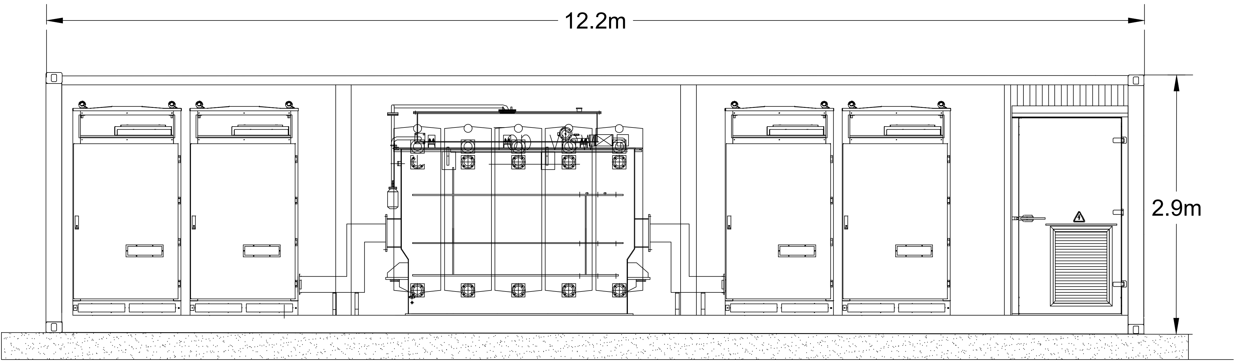
NORTHERN ELEVATION
