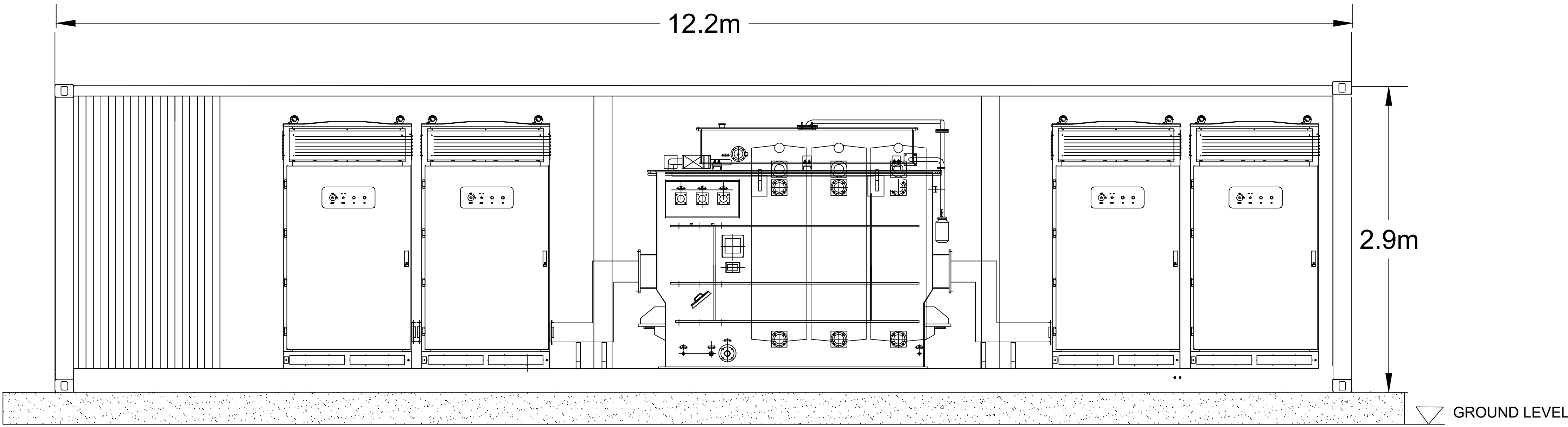
SOUTHERN ELEVATION
