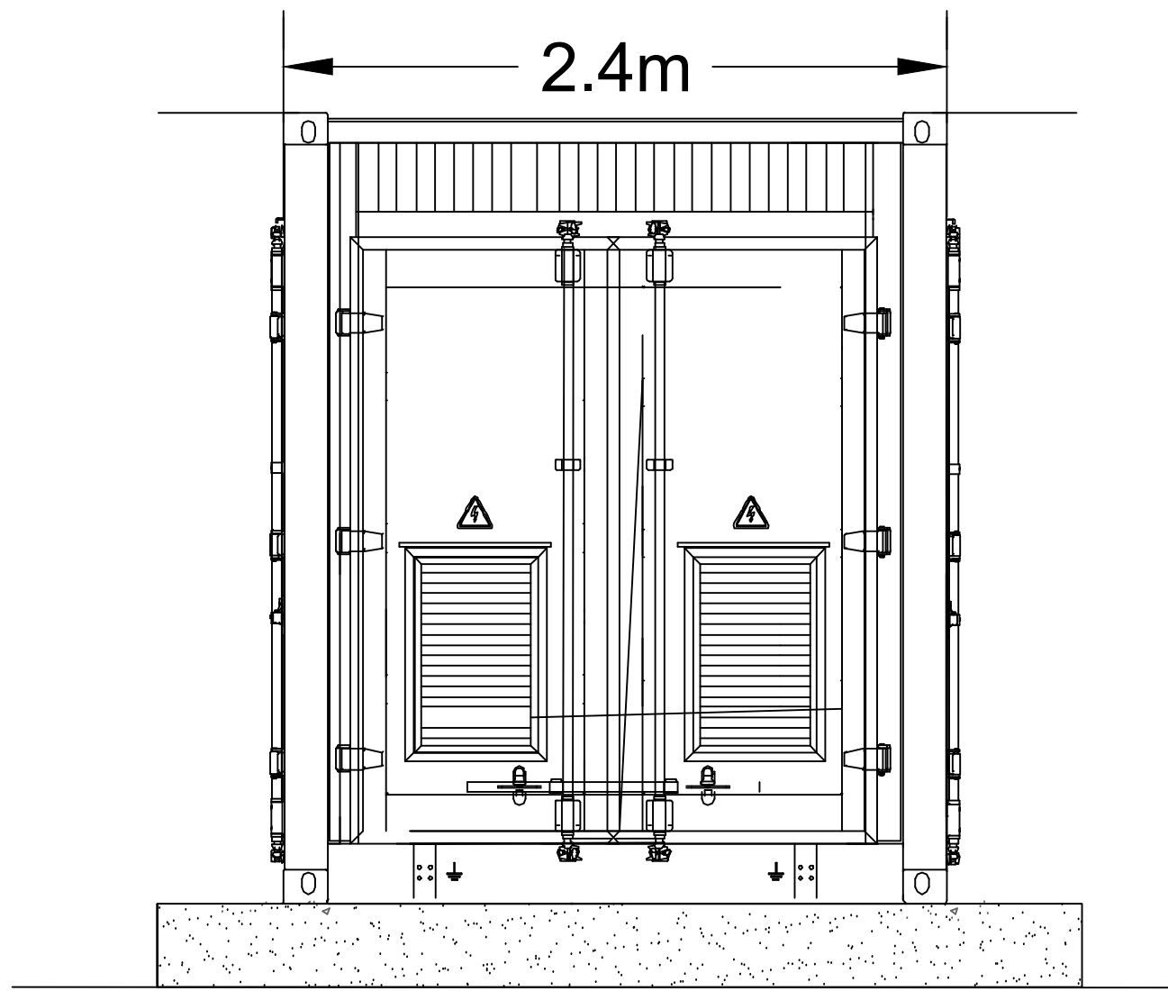
EASTERN ELEVATION
