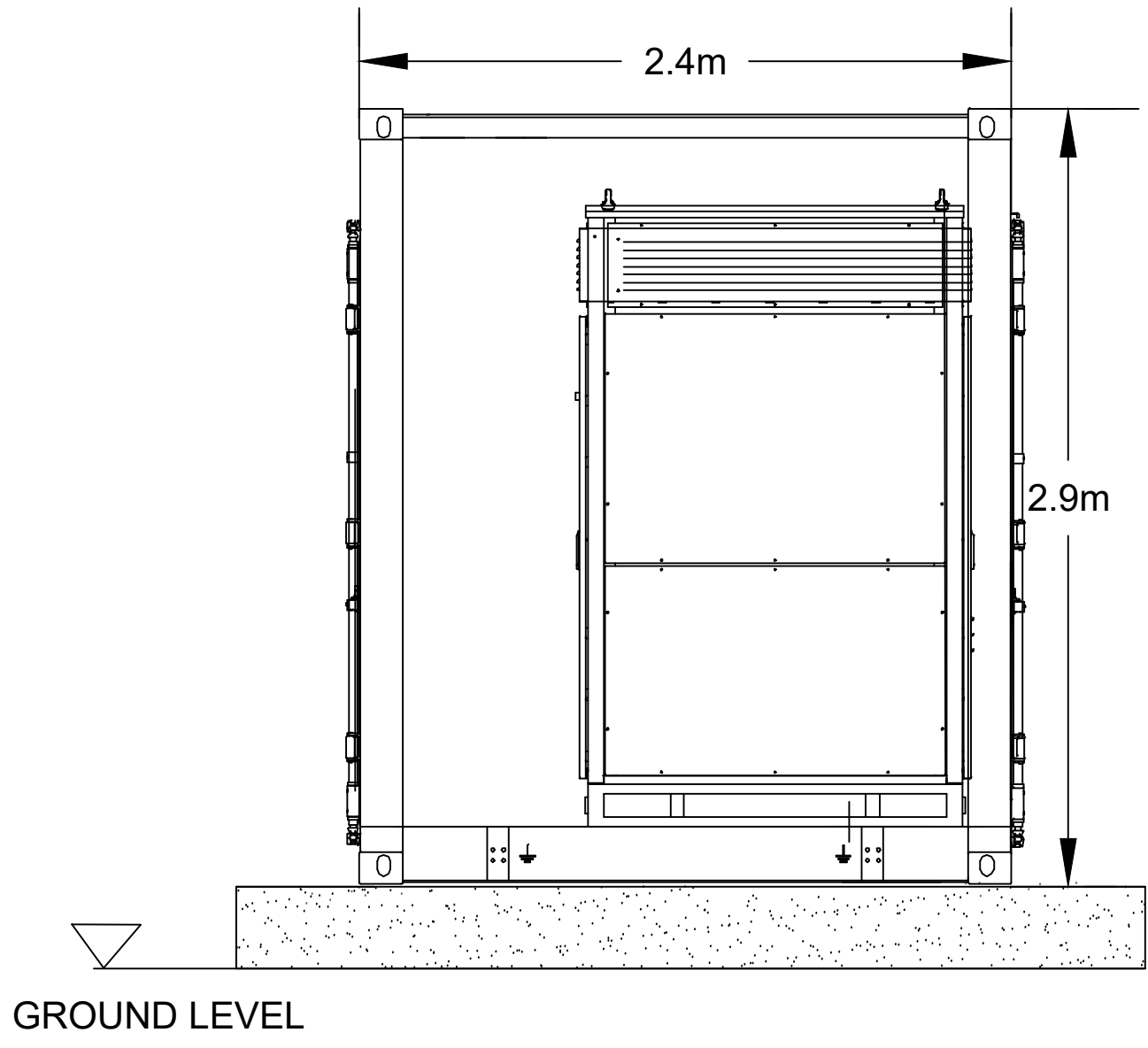
WESTERN ELEVATION
