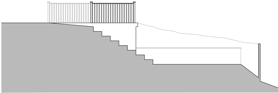
PROPOSED SIDE ELEVATION 1:100 @ A3
