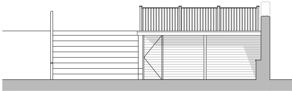
PROPOSED FRONT ELEVATION 1:100 @ A3
