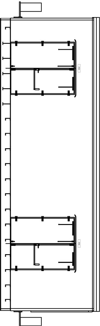
SIDE ELEVATION
