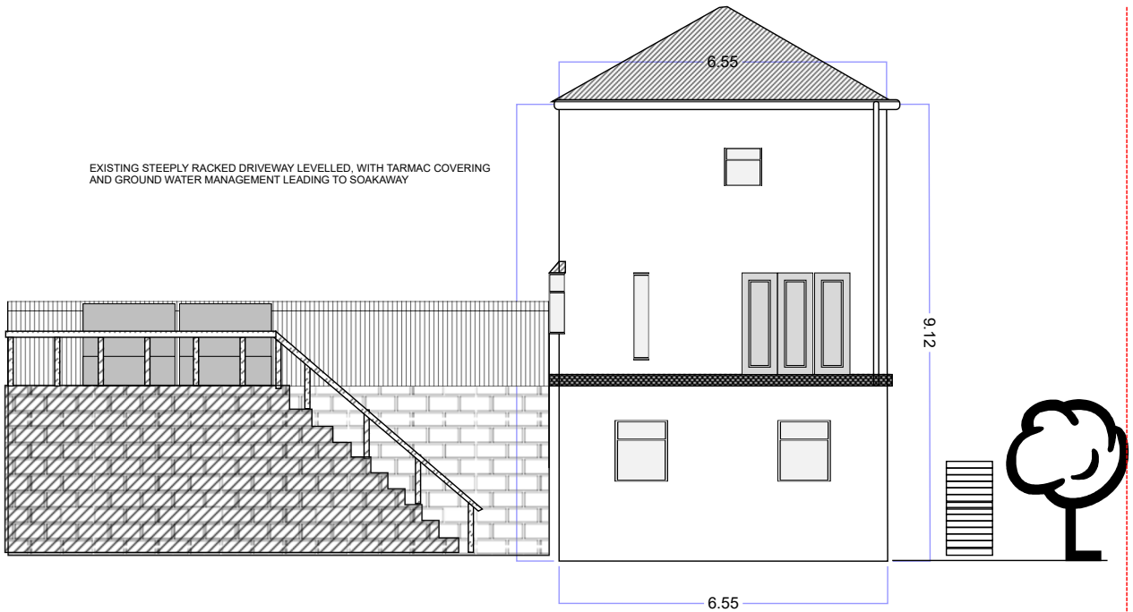
REAR (NORTH EAST) ELEVATION PROPOSED
