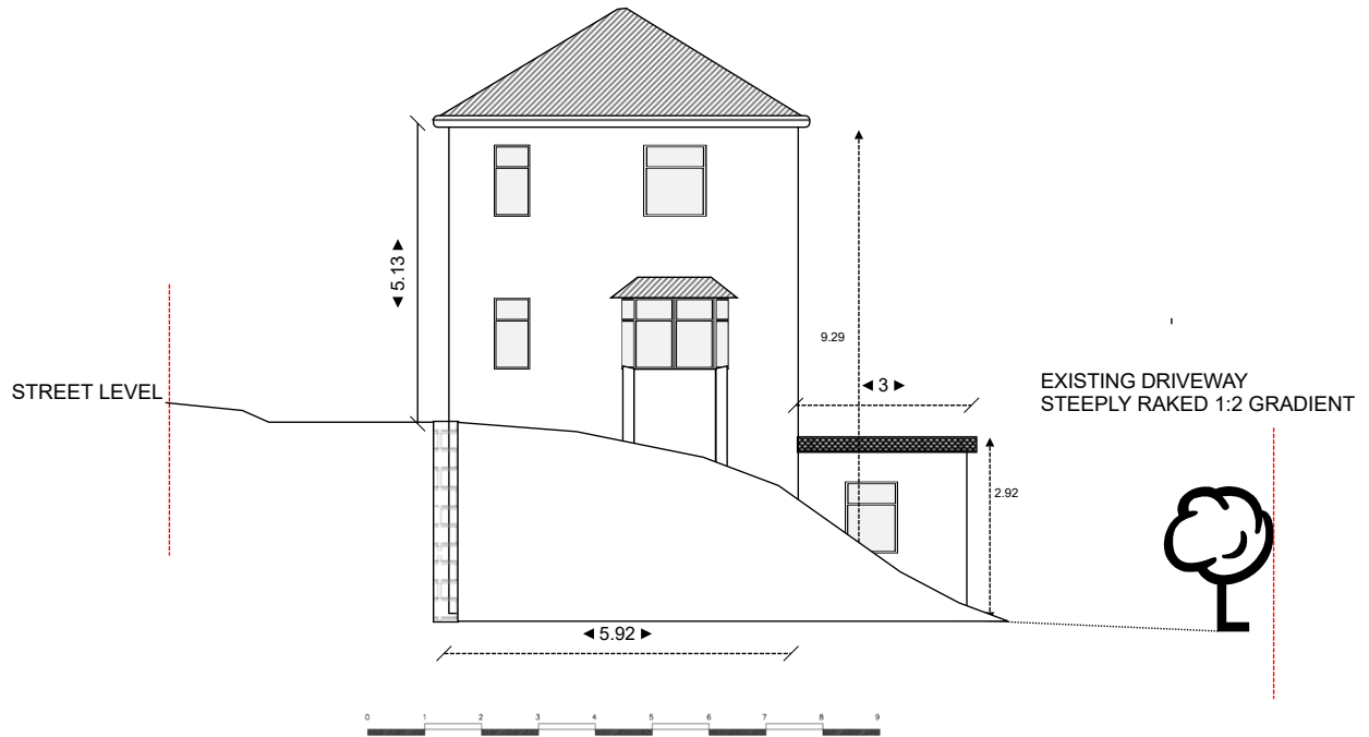
SIDE ELEVATION PROPOSED (SOUTH EAST FACE)
