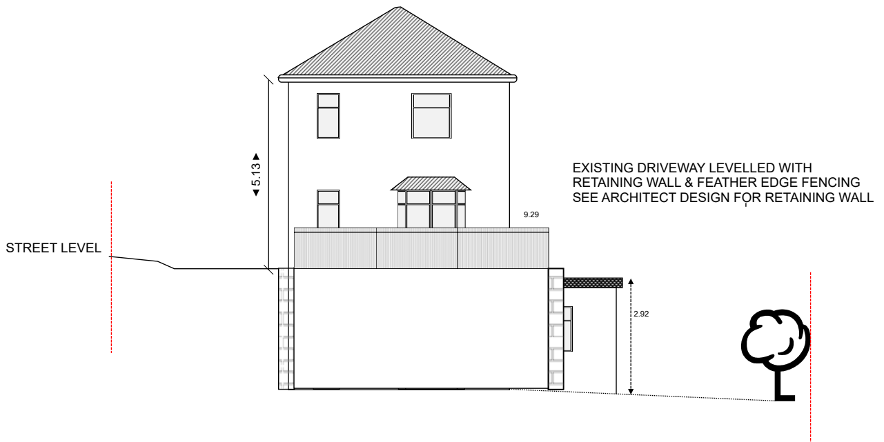
SIDE ELEVATION PROPOSED (SOUTH EAST FACE)
