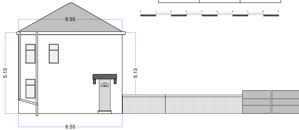
FRONT (SOUTH WEST) ELEVATION EXISTING
