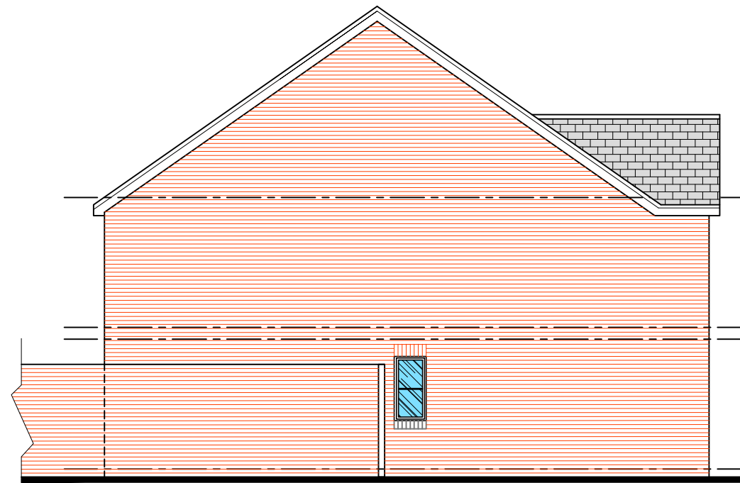
BOUNDARY WALL SIDE ELEVATION AS EXISTING
