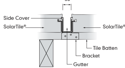
GUTTER DETAIL
