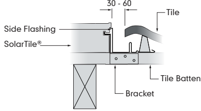
SIDE DETAIL
