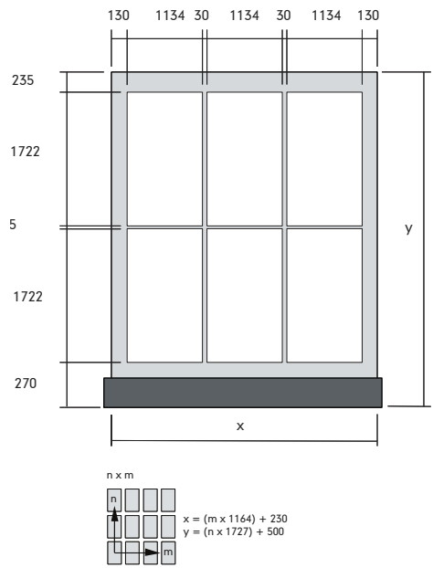
TYPICAL 405 CONFIGURATION
