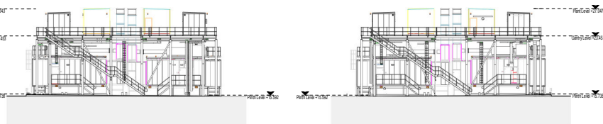
04 Generator Gantry Elevation - North 1:250
