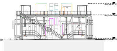
05 Generator Gantry Elevation - South 1:250
