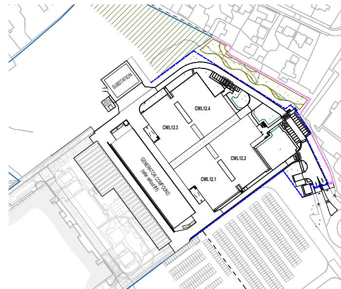
06 Security Fence Line 1:1250
