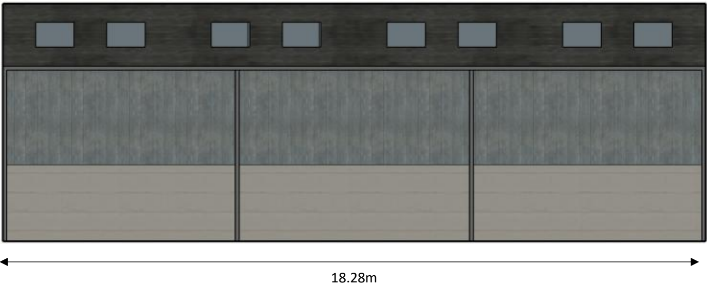
Eastern Elevation
