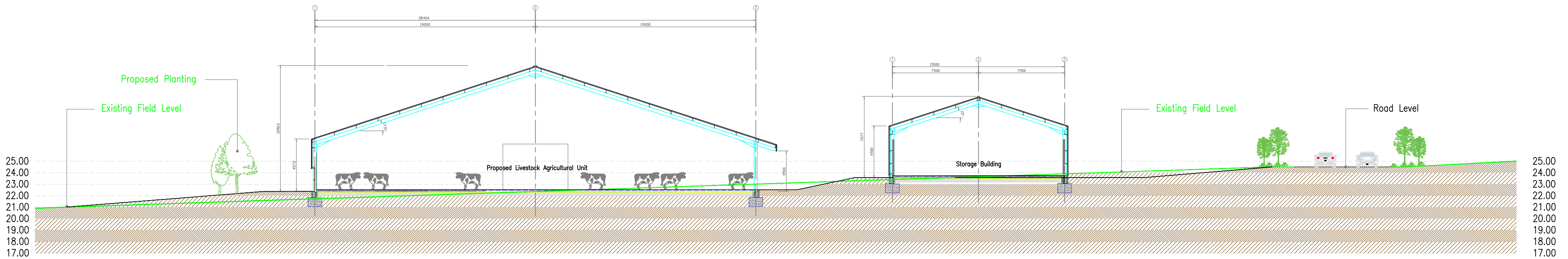
SITE SECTION A : A (North East – South West)
