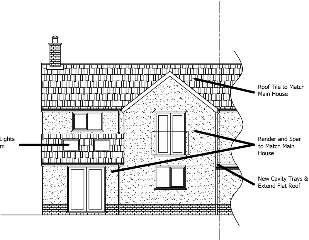
Rear Elevation
