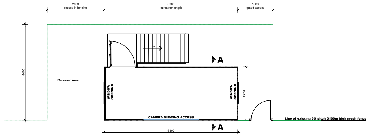
TOP CONTAINER PLAN
