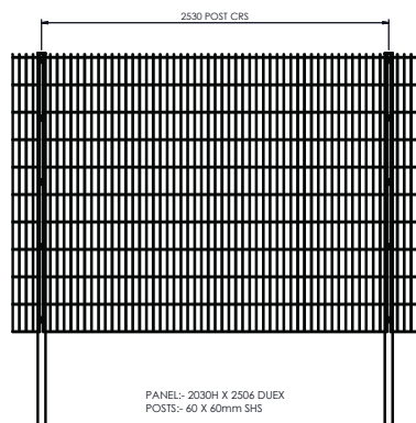
FENCE DETAILS TO MATCH EXISTING 3G PITCH FENCING (NTS)
