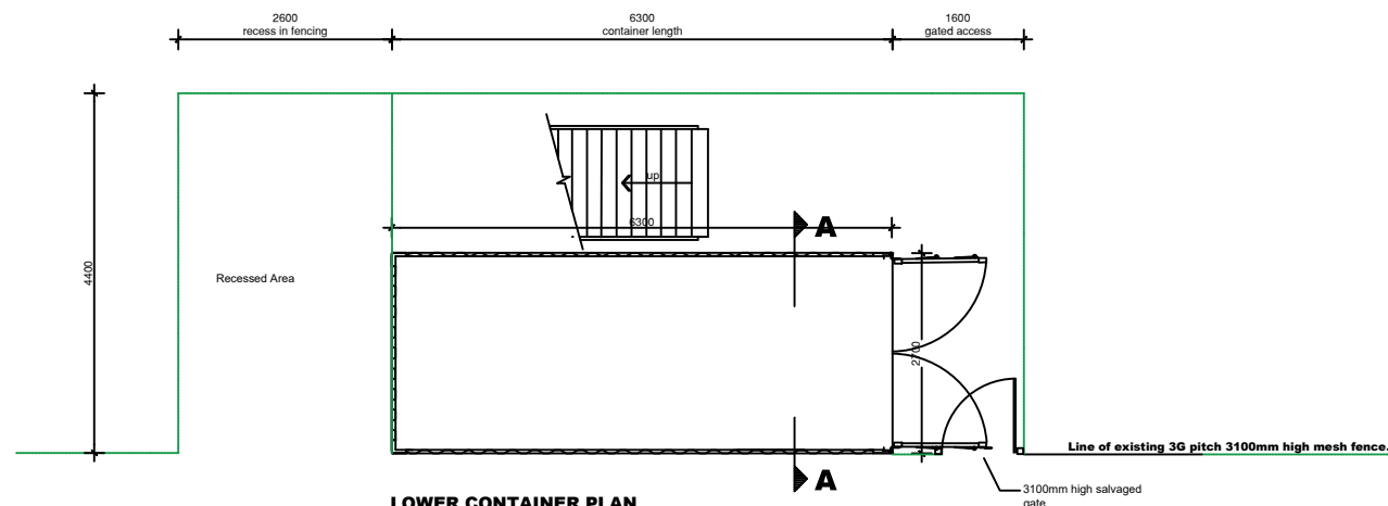
LOWER CONTAINER PLAN
