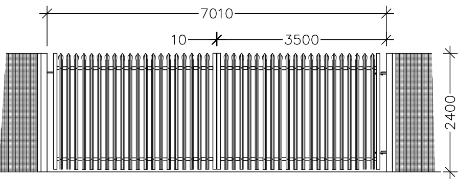
Palisade security gates
