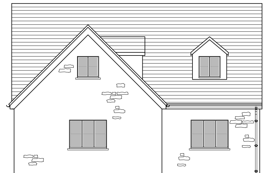
Rear Elevation
