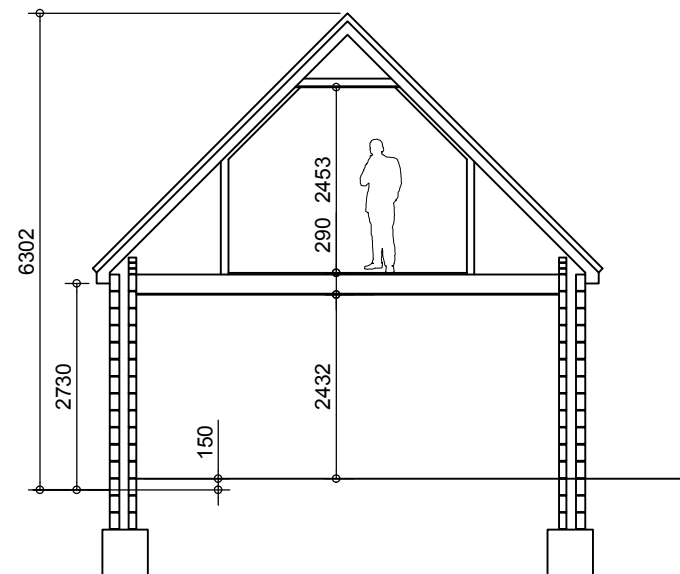
Indicative Section B-B
