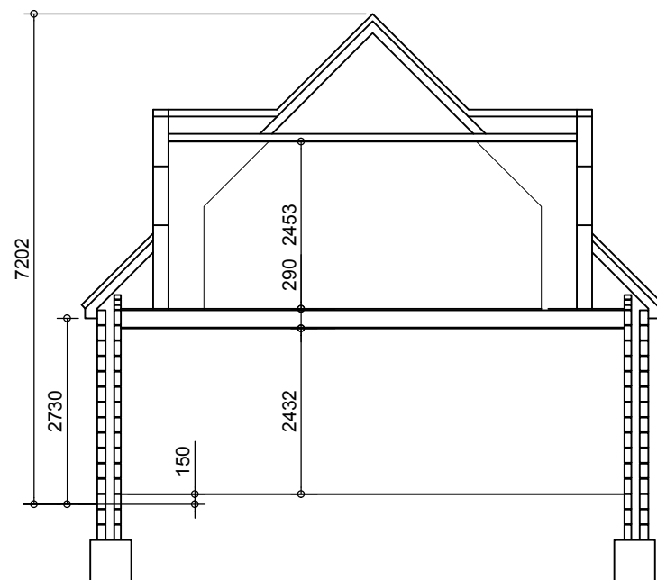
Indicative Section A-A
