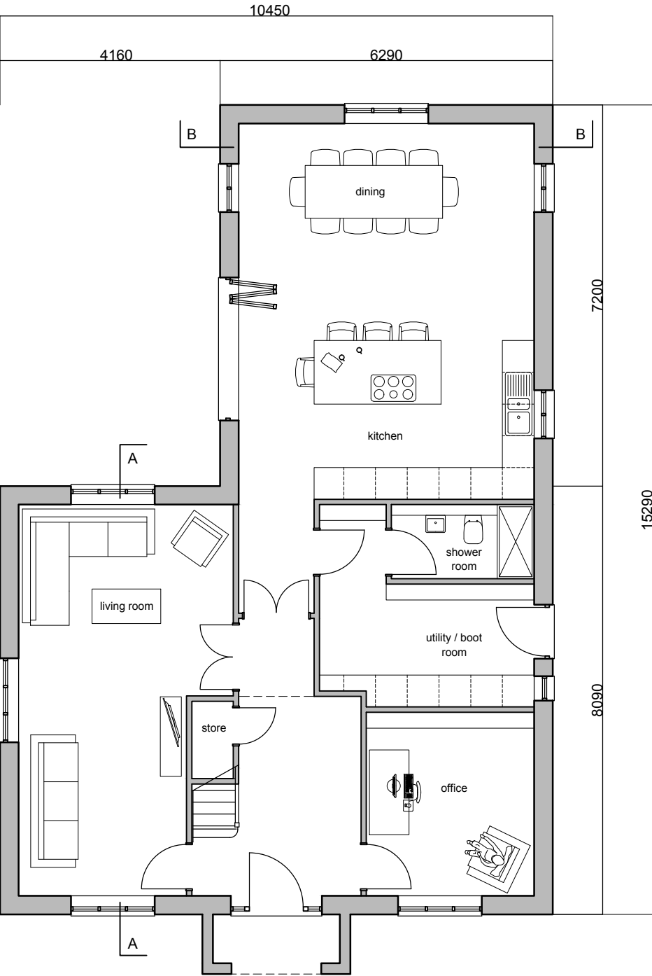
Ground Floor 1:100
