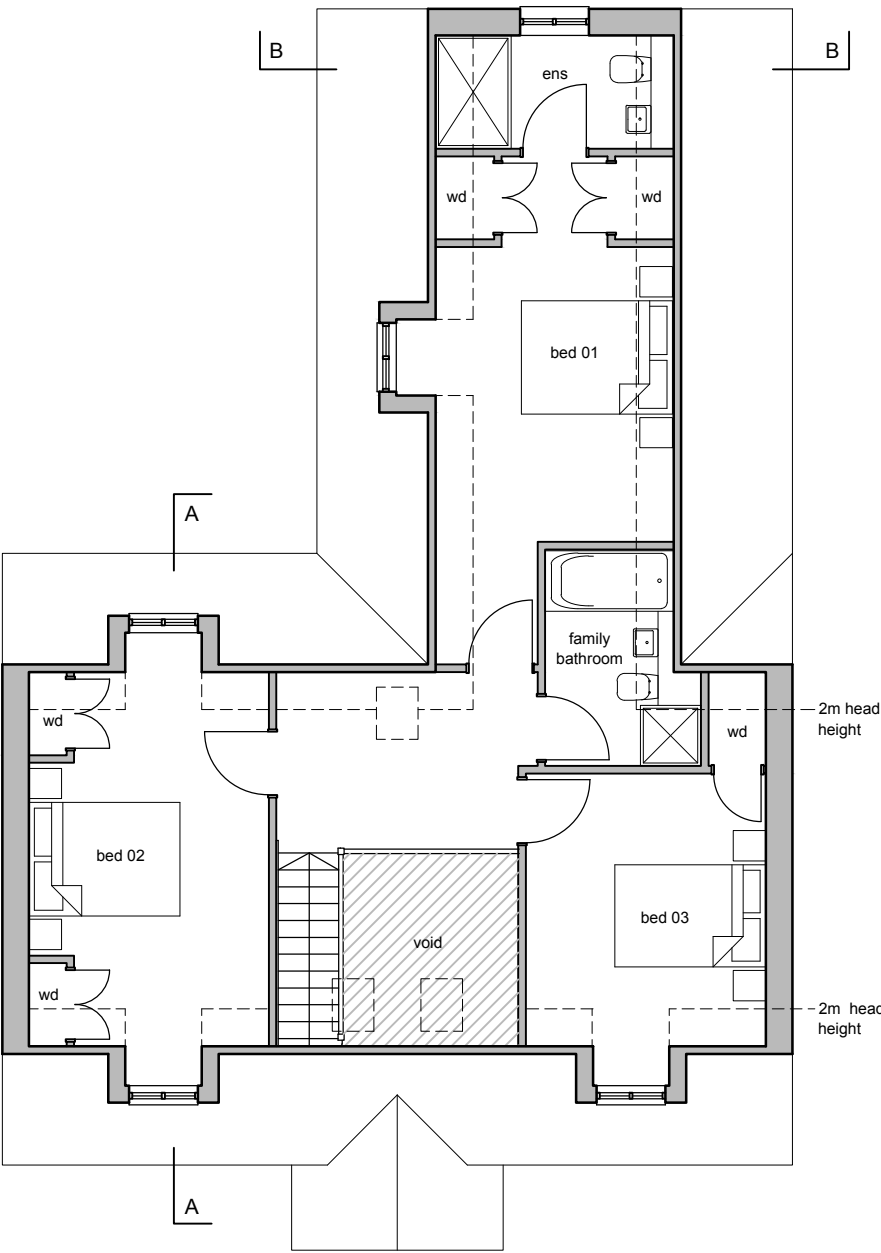
First Floor 1:100
