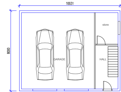
PROPOSED GARAGE GROUND FLOOR LAYOUT
