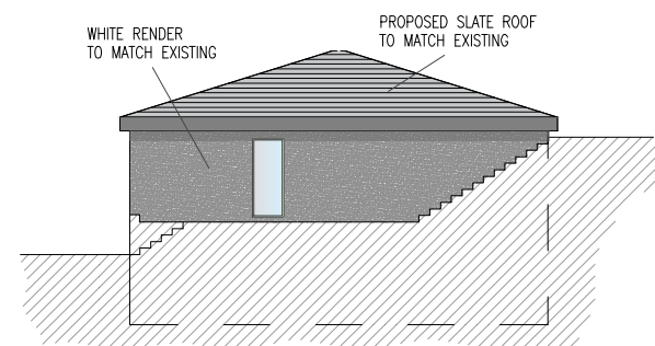
PROPOSED ANNEX SOUTHEAST SIDE ELEVATION
