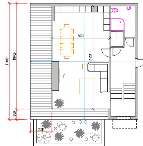
PROPOSED ANNEX FIRST FLOOR
