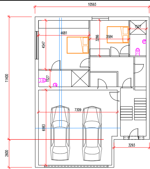
PROPOSED ANNEX GROUND FLOOR LAYOUT
