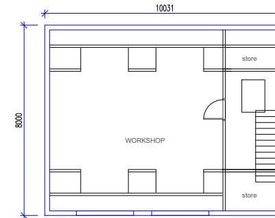
PROPOSED GARAGE FIRST FLOOR
