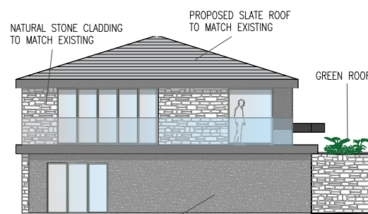
PROPOSED ANNEX NORTHWEST ELEVATION
