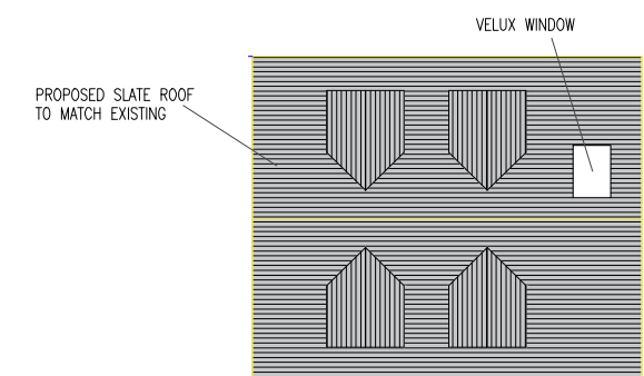
PROPOSED GARAGE ROOF LAYOUT
