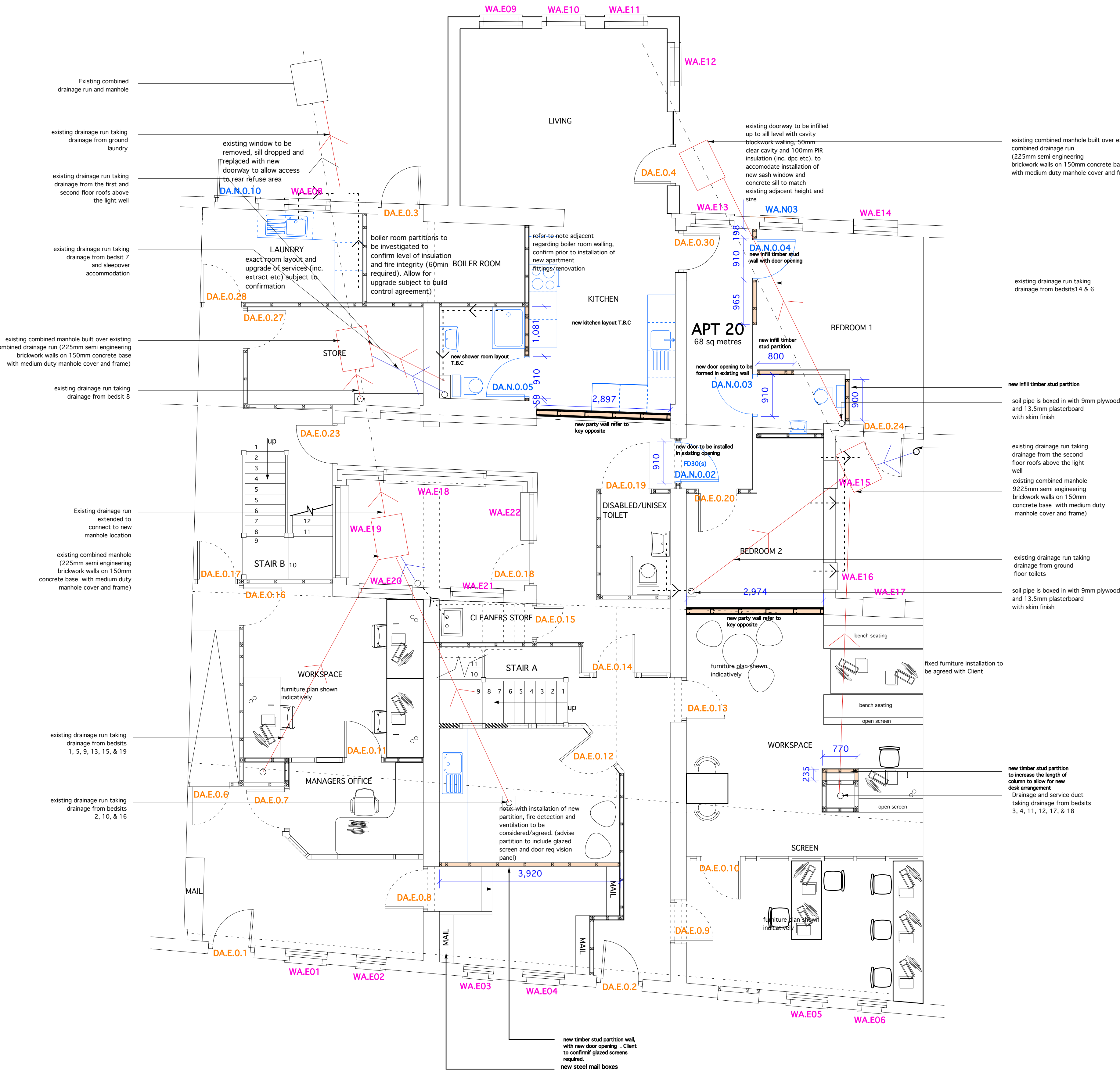
GROUND FLOOR
