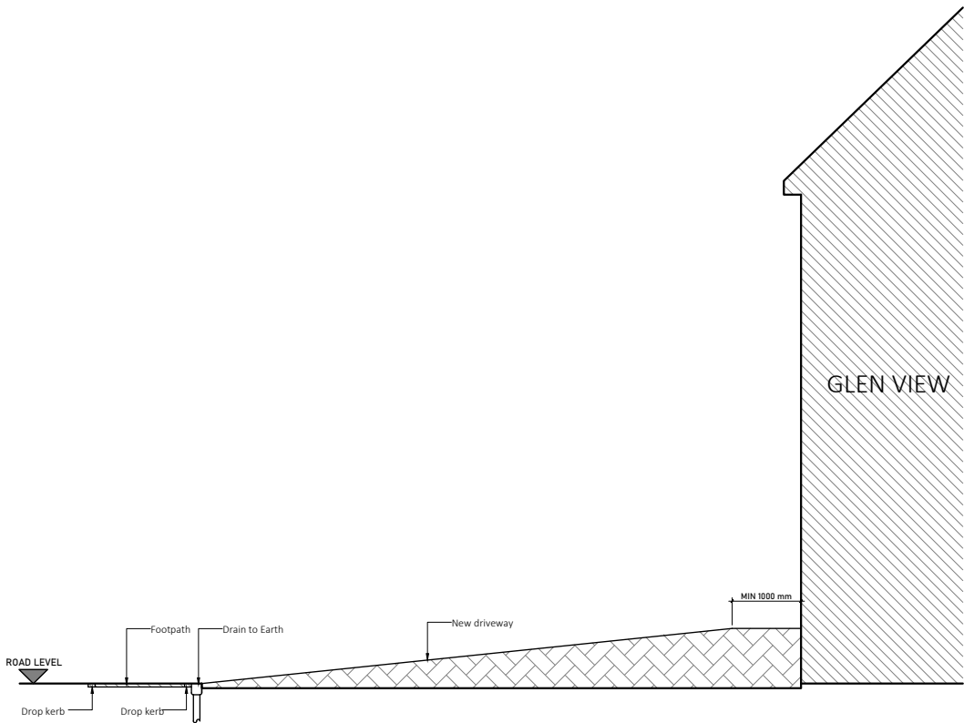
PROPOSED SECTION 1:100
