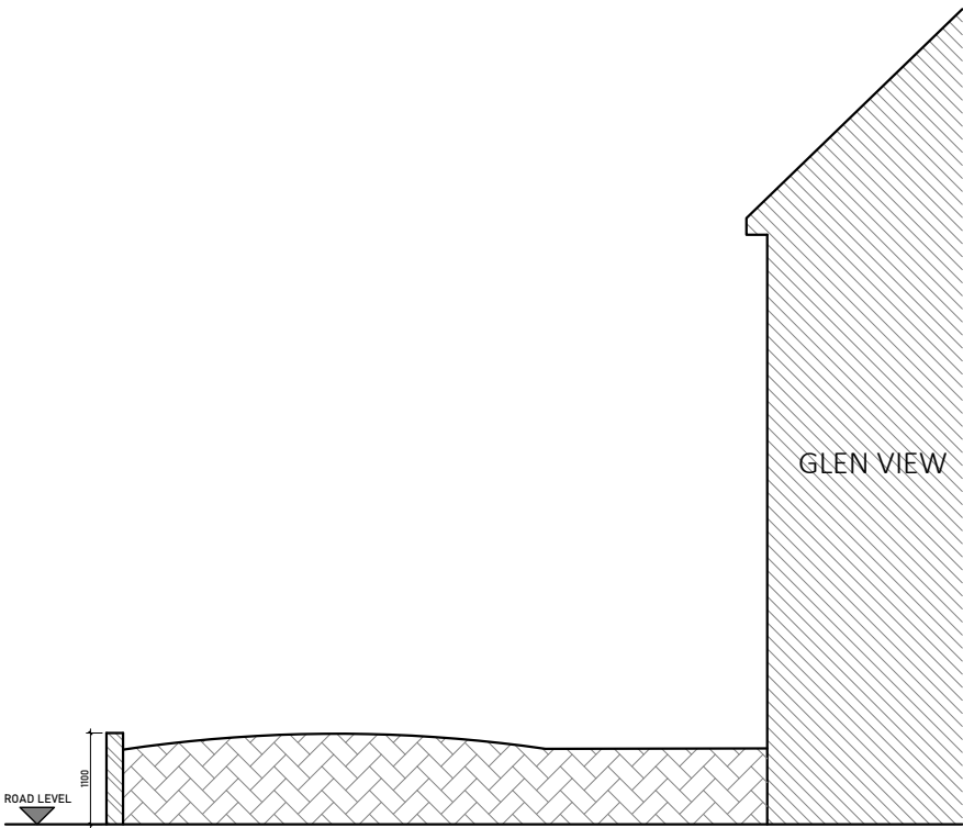
EXISTING SECTION 1:100
