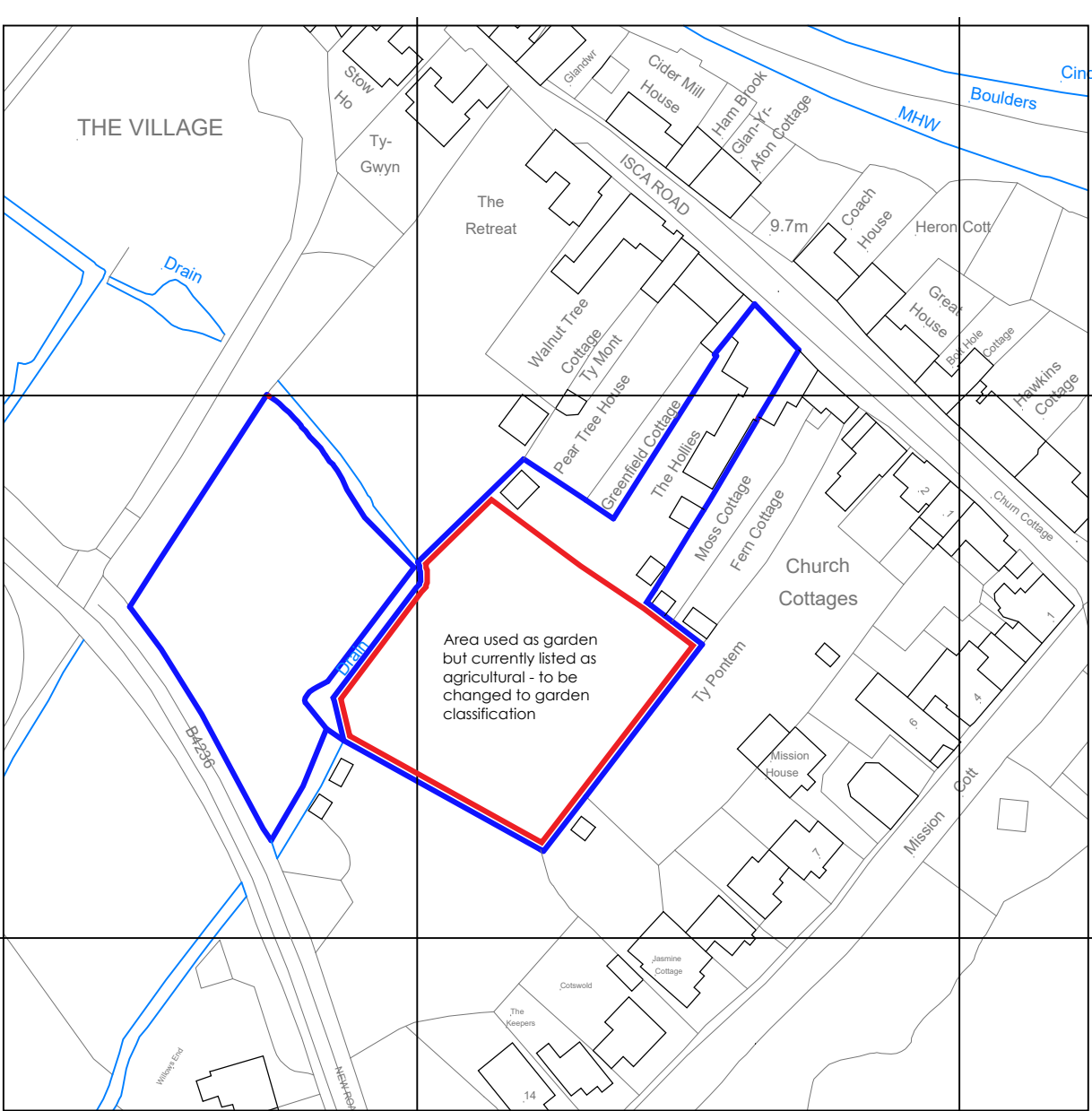
AREA OF LAND TO CHANGE USE CLASSIFICATION - 1:1250 All dimensions to be checked on site
