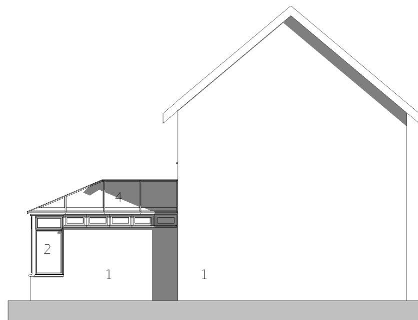
4 Side Elevation as Existing 1 1:100
