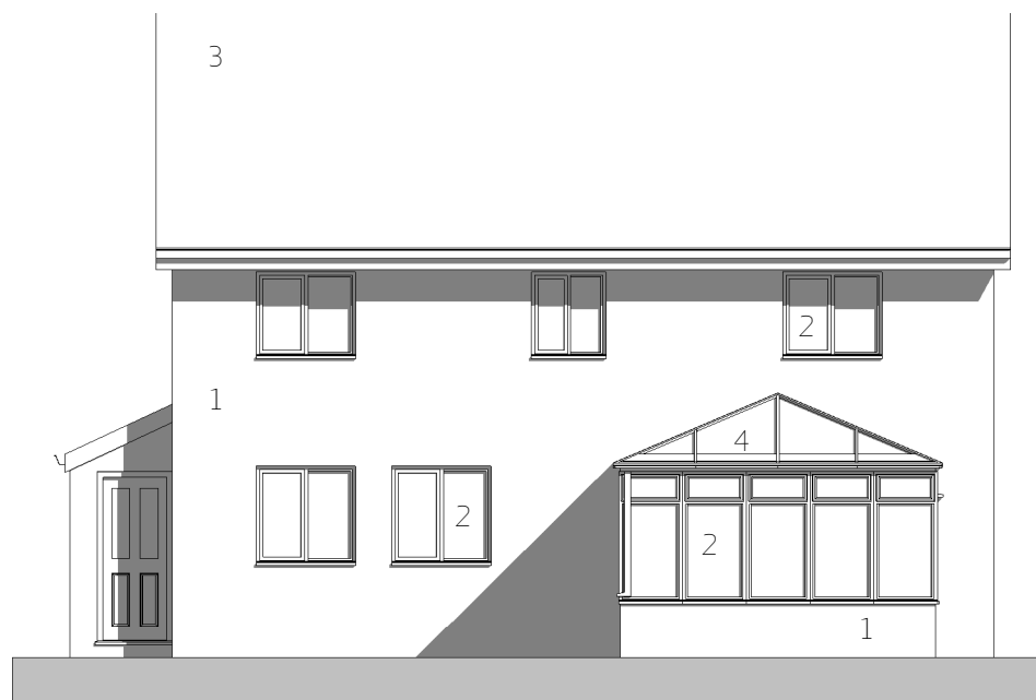
3 Rear Elevation as Existing 1:100
