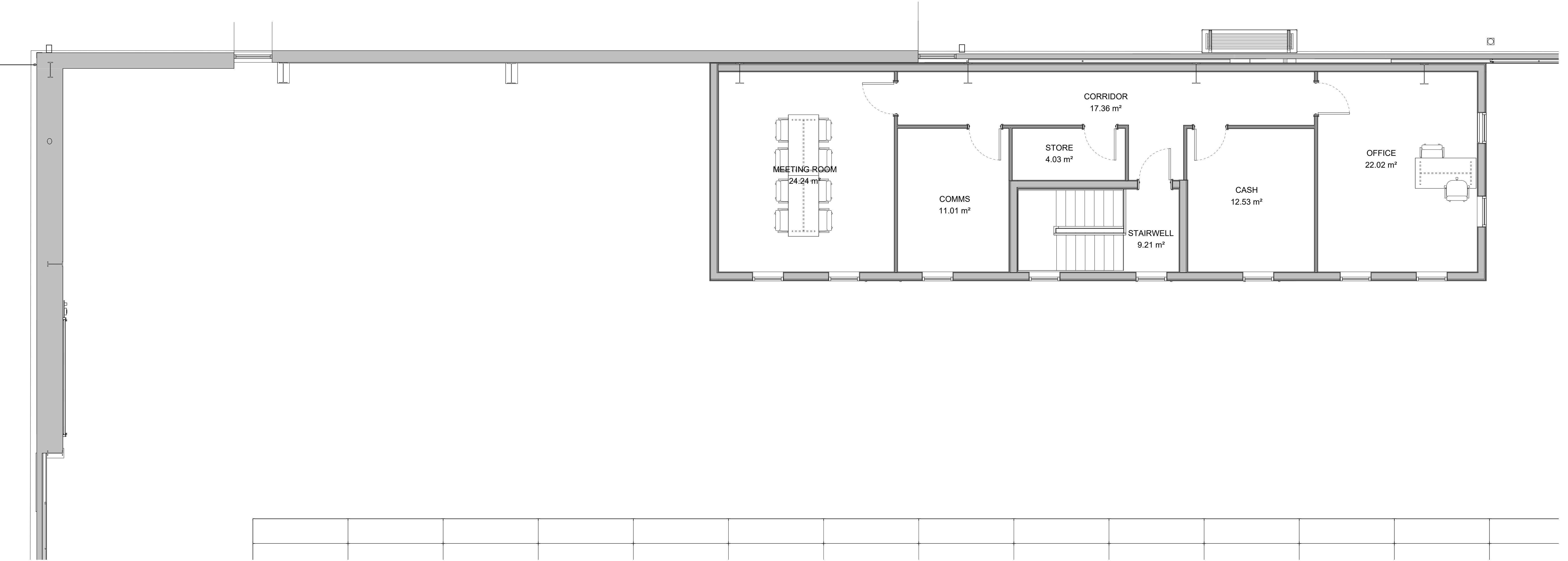
PROPOSED FIRST FLOOR - INTERNAL MEETING ROOM/ OFFICES 1 : 50
