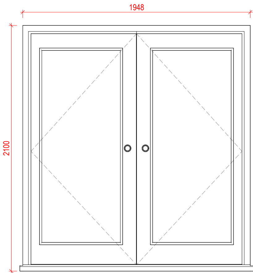
Aluminium framed entrance Double doors Black RAL 9005
