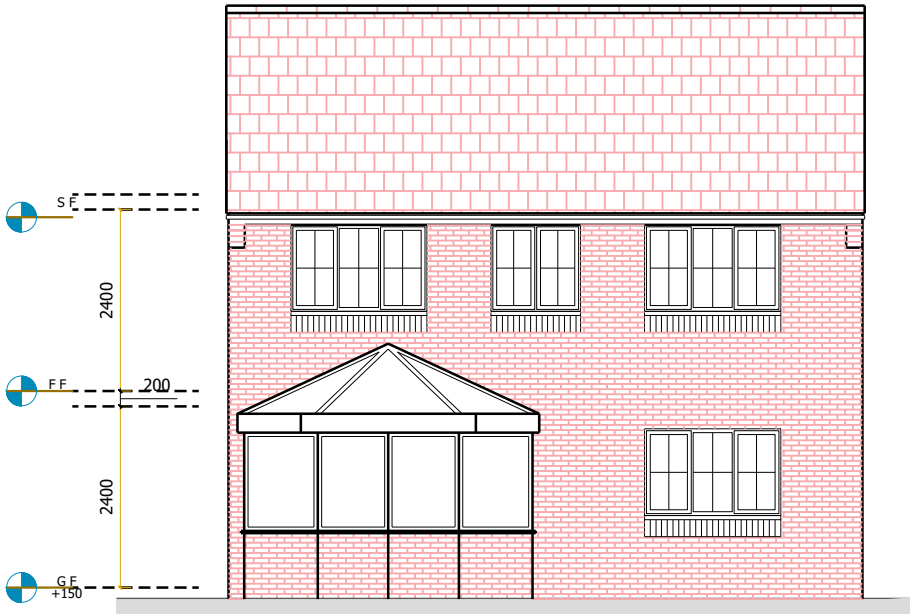
REAR ELEVATION
