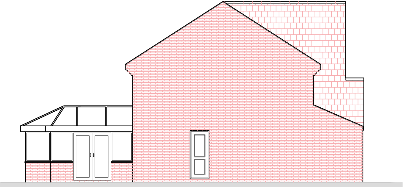
SIDE ELEVATION
