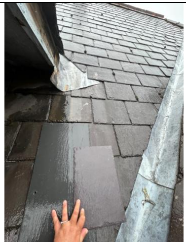
Courtyard roof – (front slope) 07.08.25 Wet conditions – NEW Glendyne and NEW penrhyn
