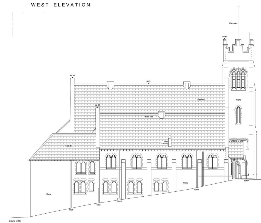
WEST ELEVATION
