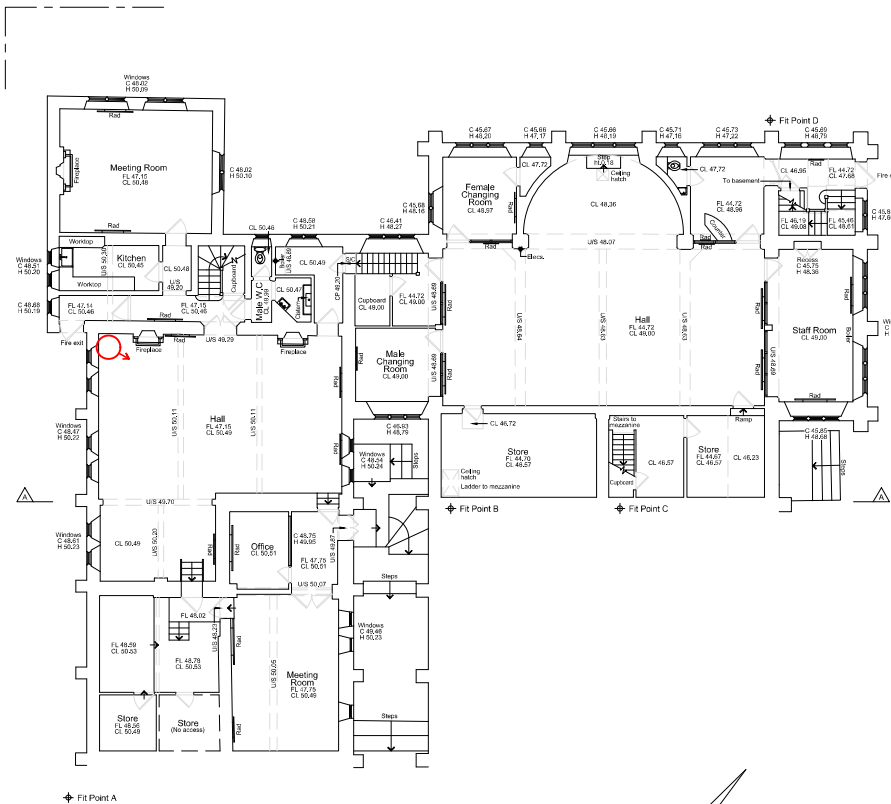
LOWER GROUND FLOOR PLAN
