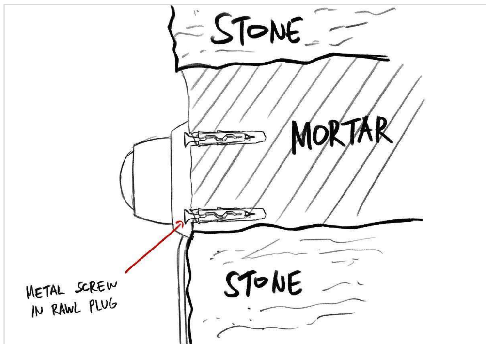
CCTV MOUNTING TO PRESERVE THE STONE
