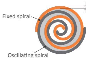
Spiral design with equal tooth thicknesses used in the conventional model
