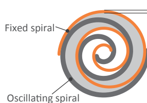
New spiral design with different tooth thicknesses
