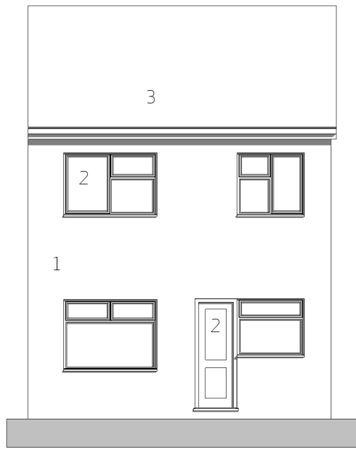
2 Rear Elevation as Existing 1:100
