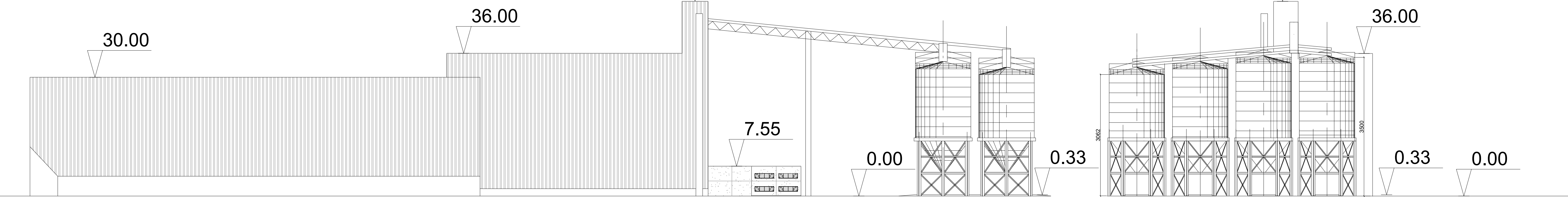
ELEVATION SOUTH
