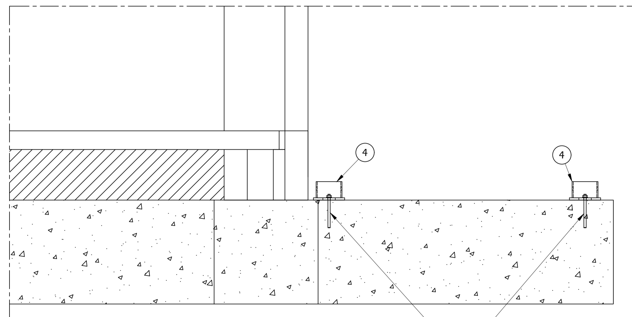
Double balcony middle pillar foot (1:10)
