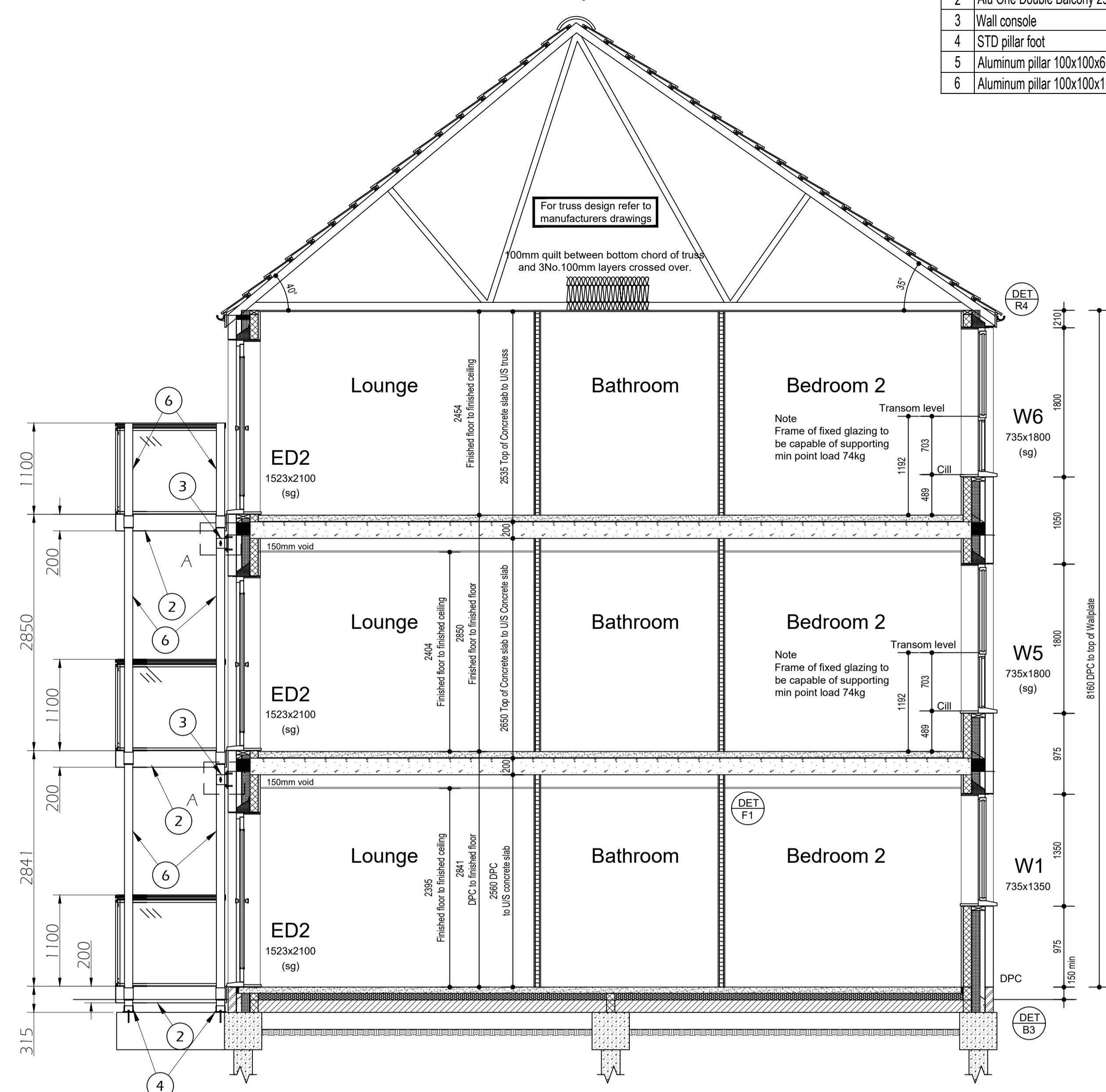
Double Balcony Middle Pillars
