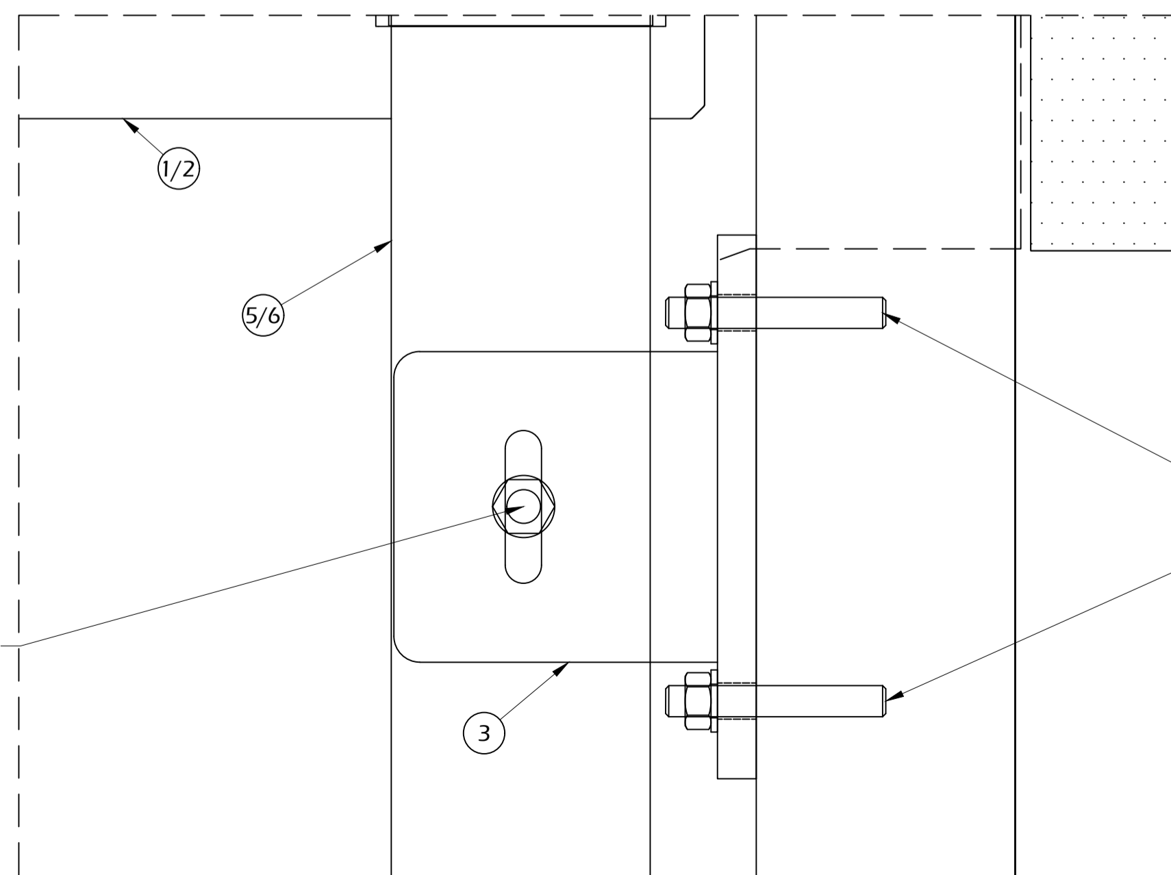
DETAIL A (1:2)
