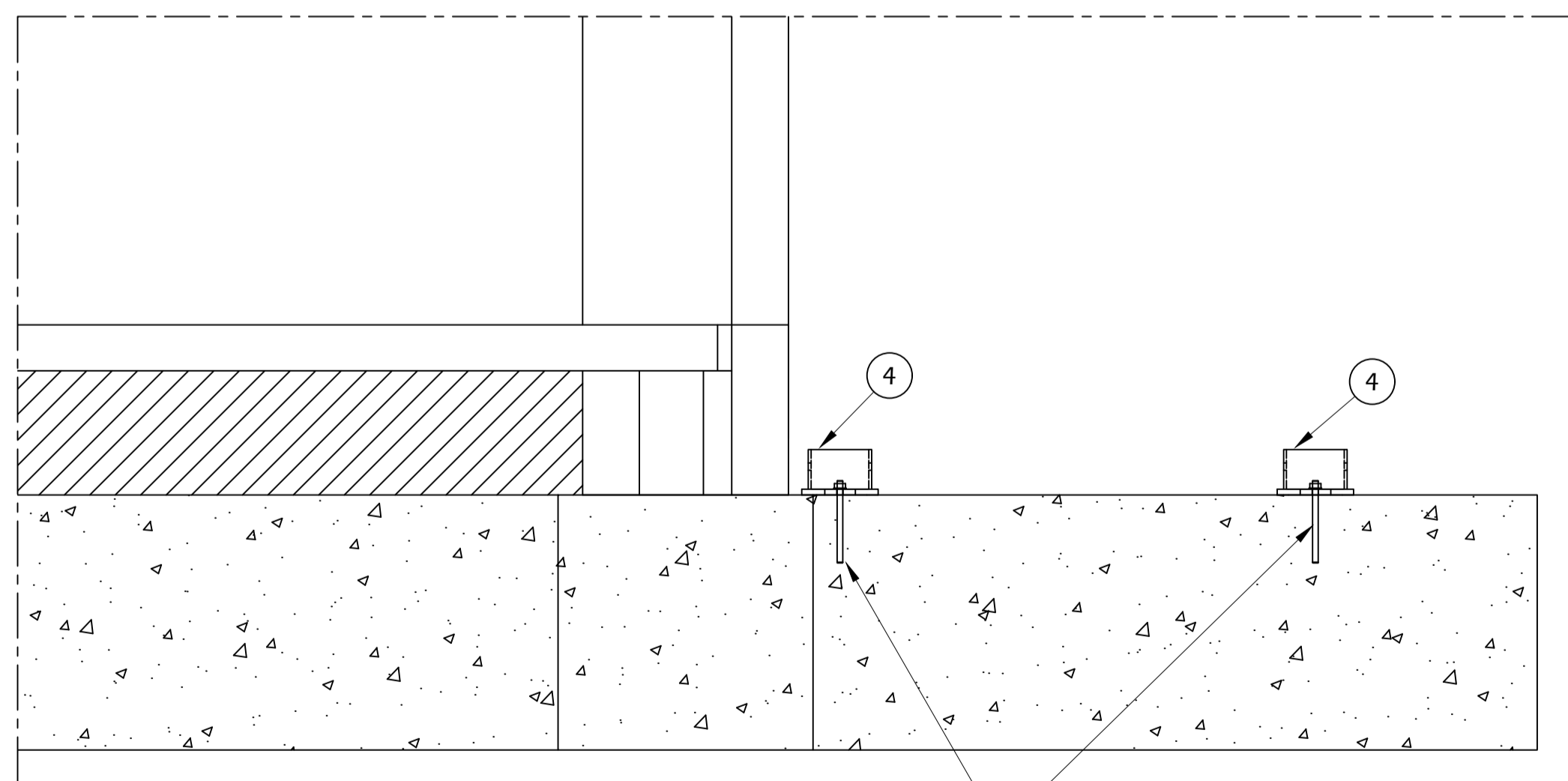
Single balcony / double balcony side pillar foot (1:10)
