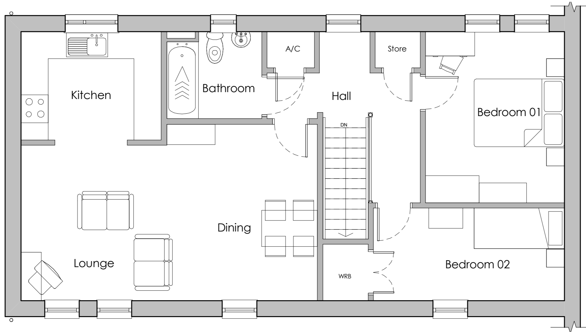
First Floor Plan House Type 'H'
