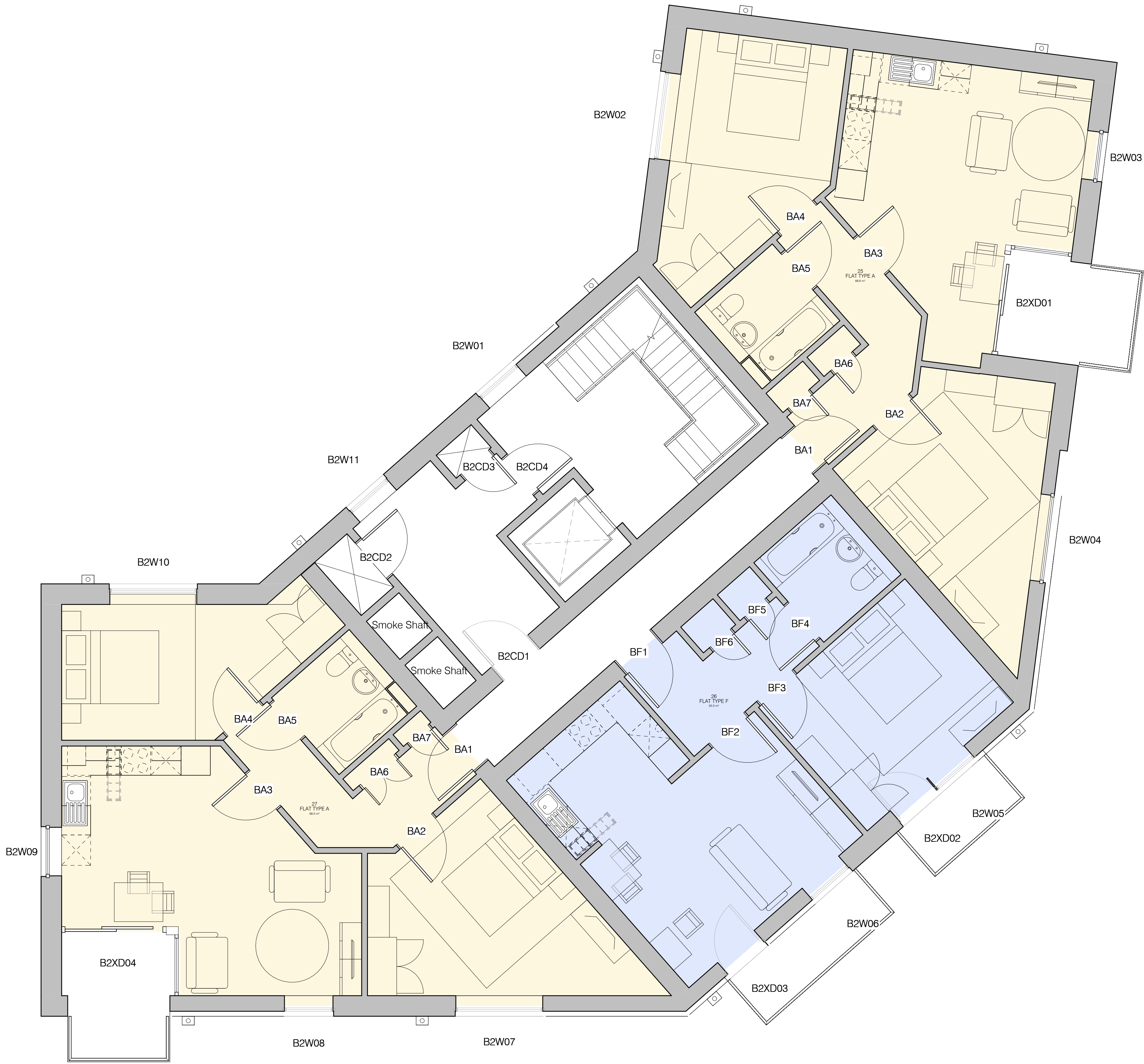
02 Second Floor GA Plan 1 : 50
