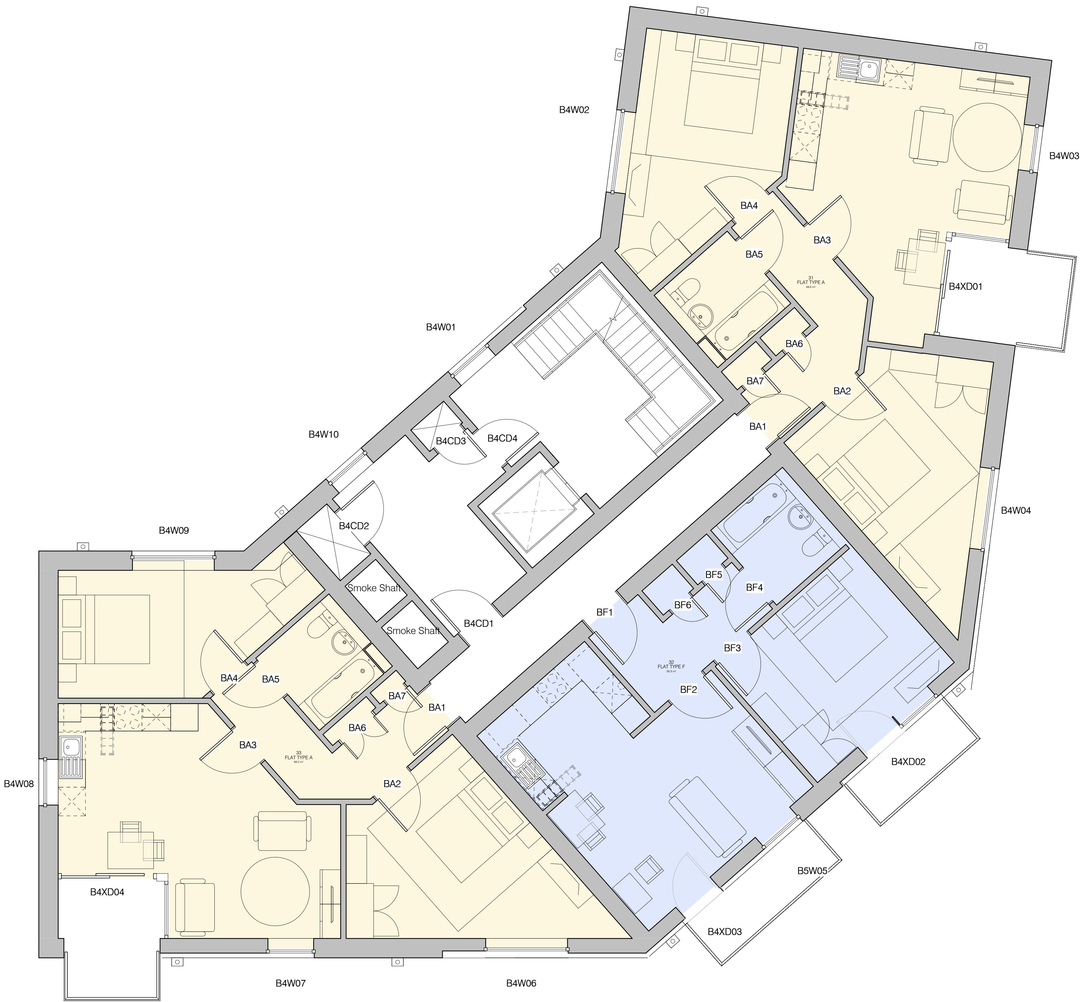
04 Fourth Floor GA Plan 1 : 50
