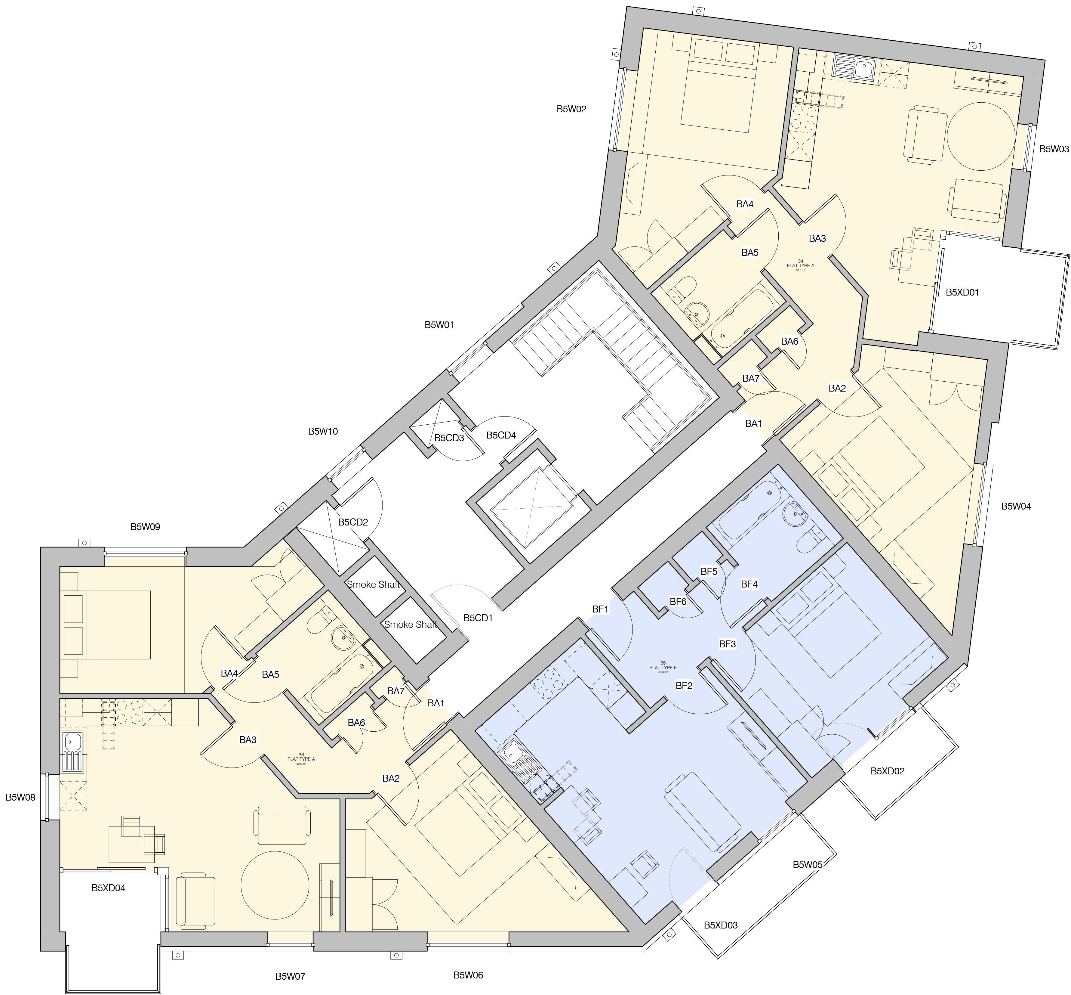
05 Fifth Floor GA Plan 1 : 50
