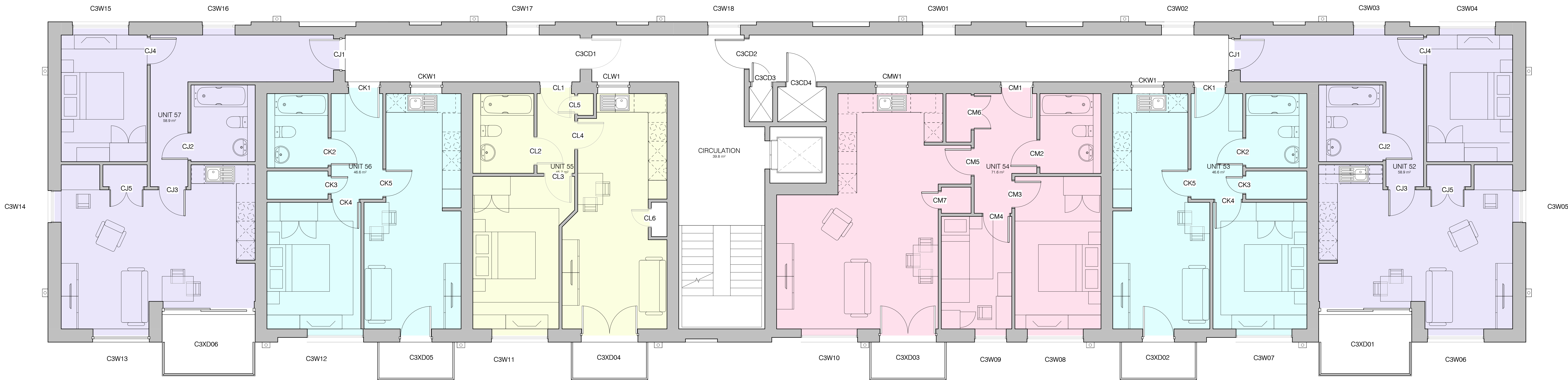
03 Third Floor GA Plan 1 : 50
