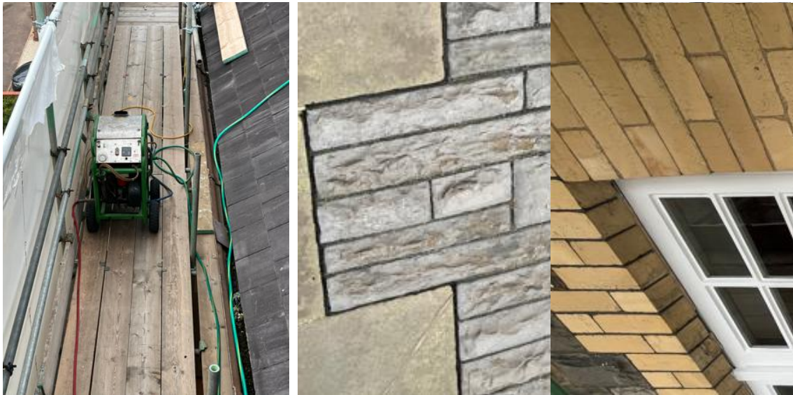
Plate 1: Thermatech Machine Plate 2 & 3: Trial section of stone and brickwork cleaned with Thermatech
