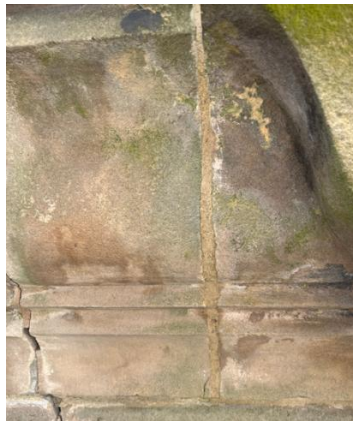
Plate 2 & 3: Trial sections of stone repointing (1:3:1 NHL2.5 /
