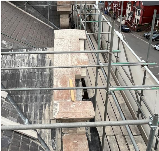
Plate 5: Cutting out defective stone (pediment 3) Templating completed for new stone order.
