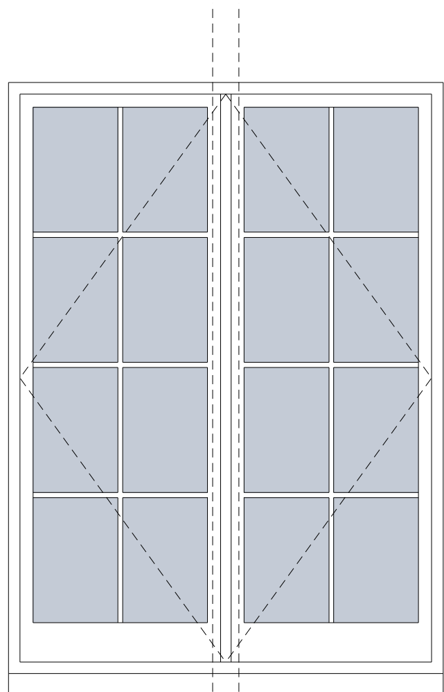
03 021 OPTION 1 - LIGHTWELL DOOR SCALE:- 1:20 AT A1
