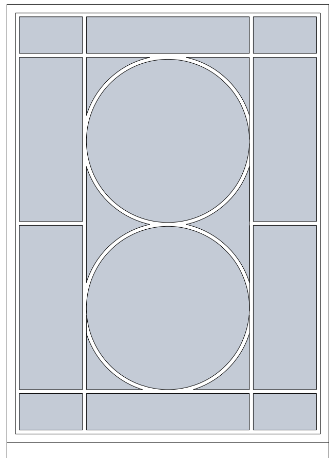
02 021 OPTION 1 - GROUND FLOOR WINDOW SCALE:- 1:20 AT A1
